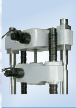
SF309 油壓拉力夾具 Hydraulic Grips
